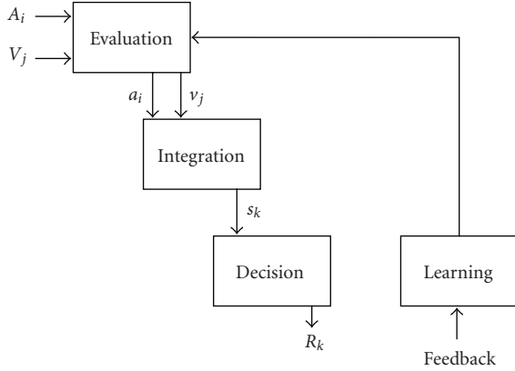
FIGURE 1: Schematic representation of the FLMP. The sources of information are represented by uppercase letters. Auditory information is represented by A_i and visual information by V_j . The evaluation process transforms these sources of information into psychological values (indicated by lowercase letters a_i and v_j ). These sources are then integrated to give an overall degree of support s_k for each speech alternative k . The decision operation maps the outputs of integration into some response alternative R_k . The response can take the form of a discrete decision or a rating of the degree to which the alternative is likely. The learning process is also included. Feedback at the learning stage is assumed to tune the prototypical values of the features used by the evaluation process.
